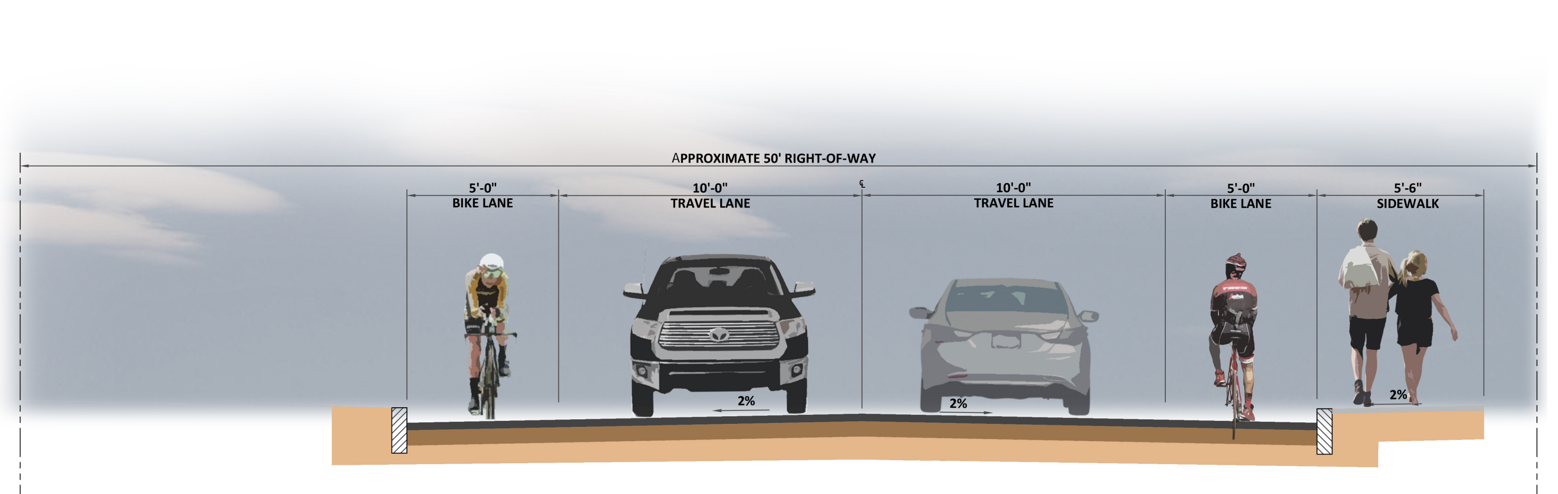
COURT STREET UNION STREET TO HUBBARD ROAD
