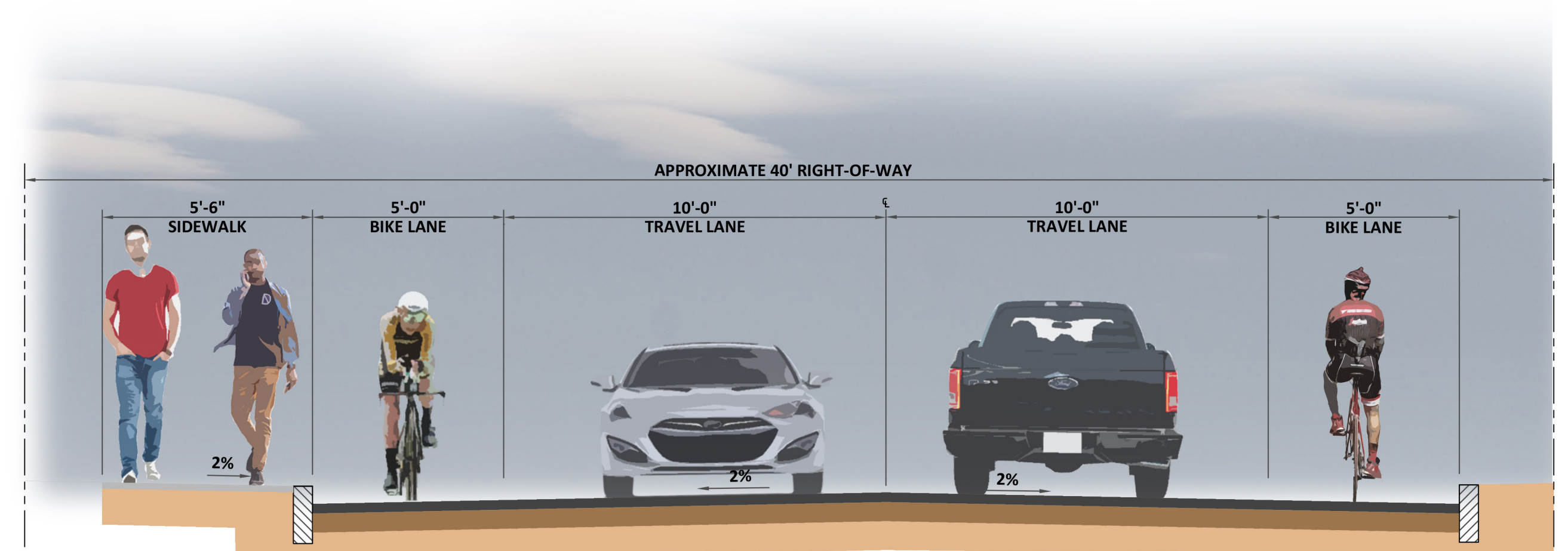
COURT STREET BOYLE STREET TO UNION STREET
