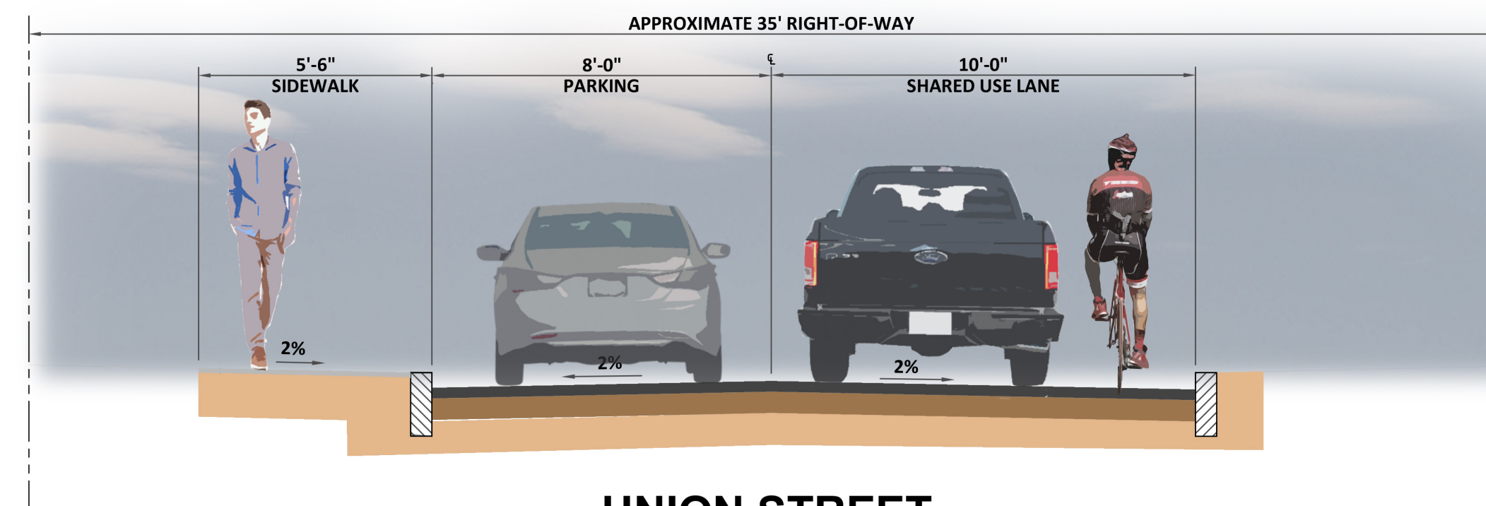
UNION STREET CENTRAL AVENUE TO COURT STREET TYPICAL SECTION
